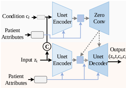
(a) Unet-based ControlNet
