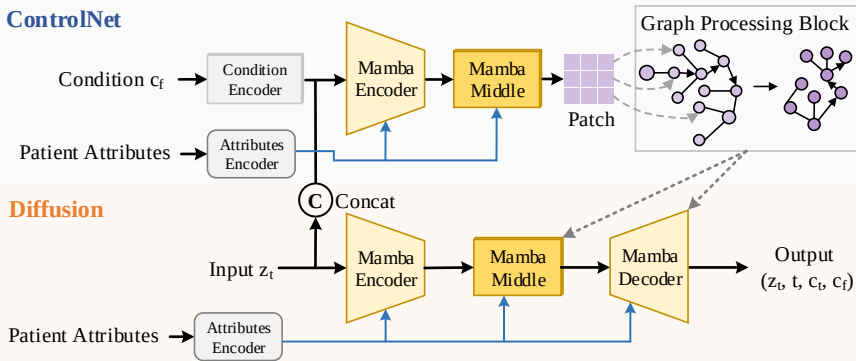
(c) MambaControl (Proposed)
