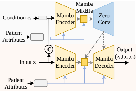
(b) Mamba-based ControlNet
